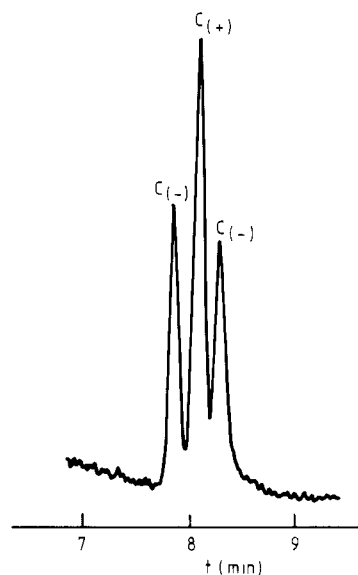
Figure 1. Gas chromatogram of soman after injection of a 1\text{-}\mu\text{L} sample of a 4\text{-mM} solution of soman in i -PrOH on a Chirasil-Val column ( l = 25 \text{ m} , \phi = 0.3 \text{ mm} ; plate number 3 \times 10^4 , peak 1), column temperature 80 \text{ }^\circ\text{C} , precolumn pressure 103 \text{ kPa} , injection split ratio 1:10. The injection block and the FID-detector block of the Pye-104 gas chromatograph were held at 300 \text{ }^\circ\text{C} .
