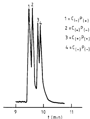
Figure 2. Gas chromatogram of soman on a Carbowax 20M/Chirasil-Val column. The Carbowax 20M column ( l = 30 \text{ m} , \phi = 0.3 \text{ mm} ) was coupled directly to the same Chirasil-Val column as described in Figure 1. The Carbowax leg of the system was connected with the injection port of the gas chromatograph. The theoretical number of plates of the combined column is 1.3 \times 10^5 (peak 1). See Figure 1 for further chromatographic conditions.
